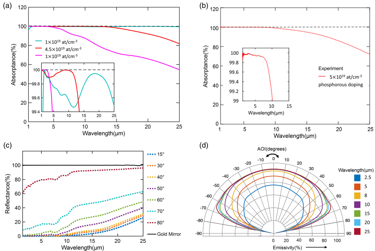
Figure 5. The doping level of silicon as the second key parameter to achieve ultrabroadband and ultrablack silicon. a) Calculated absorptance over the infrared spectral range from 1 to 25 μm for different values of the doping level of N-type, phosphorous-doped silicon with fixed average cone depth \langle d \rangle = 10 \mu\text{m} . The inset gives a zoom on the vertical scale to highlight that widest spectral ranges achieved at moderate doping level 1 \times 10^{19} \text{cm}^{-3} also correspond to the smallest levels of absorptance, although still high; higher absorptance is attainable at higher doping levels but at the expense of a reduced spectral range. b) Experimental spectral absorptance of black silicon for high ( 5 \times 10^{19} \text{cm}^{-2} ) doping level measured over the spectral range from 1 to 25 μm, showing excellent agreement with simulation. c) Reflectance of black silicon for high ( 5 \times 10^{19} \text{cm}^{-3} ) doping level measured reflectance at different incident angles, and d) corresponding emissivity diagrams.
