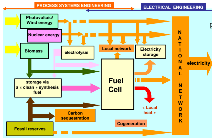
Fig. 1. The fuel cell example: the core of a future energy portfolio mixing electrical engineering and process systems engineering disciplines.
