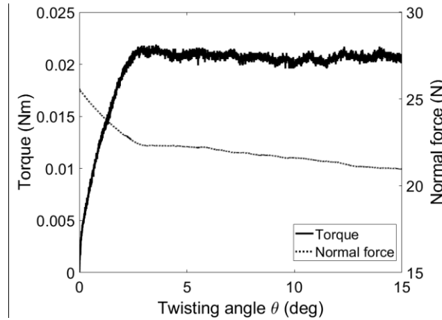
Fig. 2: Evolution of the experimental torque (plain line) and normal force (dotted line) as a function of the twisting angle for a typical friction test.
