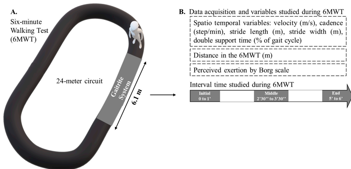
Figure 1. (A) gait evaluation during the six-minute walk test (6MWT); (B) variables studied during each interval of the 6MWT [25].
