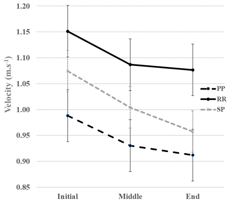
Figure 5. Variations of the velocity during the 6MWT for PwMS with PP, RR, and SP phenotypes. PP, Primary Progressive; RR, Relapsing–remitting; SP, Secondary Progressive.
