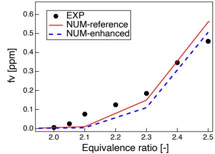
Figure 8: Comparison between experimental [20] (symbols) and numerical f_v for \phi at a distance of 15 mm from the flame front with the reference (continuous) and the enhanced (dashed) oxidation model in a laminar premixed flame at ambient temperature and atmospheric pressure for different \phi .
