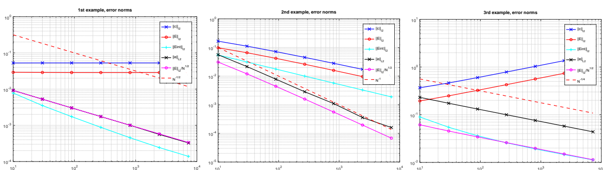
FIGURE 3. Error norms, compared to N^{-1/2} (Ex. 1), N^{-1} (Ex. 2), N^{-1/4} (Ex. 3),
