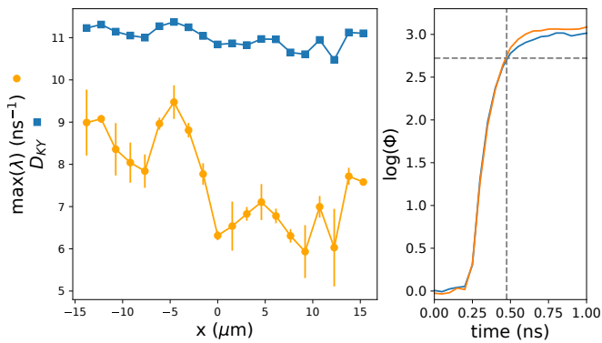
Figure 2. a) Largest Lyapunov exponent \lambda_M = \max(\lambda) and Kaplan-Yorke dimension D_{KY} of the time traces versus recording position. b) Initial error growth rate for the laser intensity versus time computed at C for both photodetector recordings. The extracted prediction time horizon (see text) is 0.47 ns.
