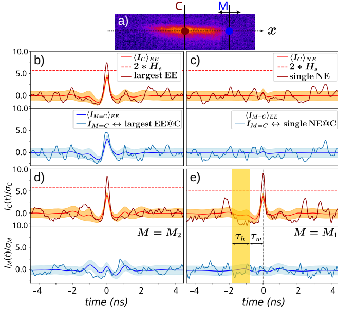
Figure 1. a) Microlaser near-field image above lasing threshold. b-e) simultaneous recording of scaled intensities at C (fixed photodetector, upper) and M (mobile photodetector, lower) for specific events at C (placed at t = 0 ): an EE is present (b,d,e) or not present (c) at C. The photodetector is located at x_M = 0 \mu\text{m} in b), x_{M_2} = +12.3 \mu\text{m} in d) and x_{M_1} = -13.8 \mu\text{m} in e). Red and black lines: average time-traces over the ensemble of EE or NE and associated standard deviations (orange and light blue shaded areas). Dark red: largest EE's timetrace, in b,d,e, (resp. single random NE in c) recorded at C with the simultaneous timetrace recorded at M (light blue). Red dashed line: EE threshold 2 * H_s (to be compared to the pulse height H from the trough to peak, not to the peak value). Yellow shaded area in e): information used for the prediction of an event at t = 0 , with history time \tau_h and warning time \tau_w .
