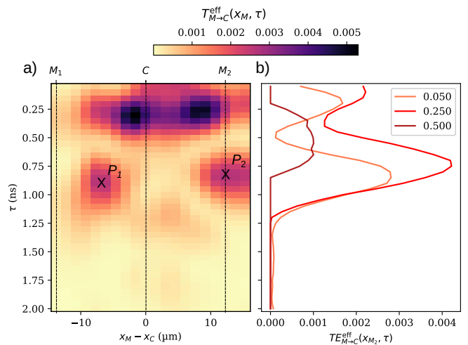
Figure 3. Effective transfer entropy T_{M \rightarrow C}^{\text{eff}} as a function of x_M and delay \tau for \tau_h = 1\Delta t = 0.050 ns and b) at M_2 for \tau_h = 0.050, 0.250, 0.500 ns. P_1 and P_2 locate the main precursor regions in the spatiotemporal diagram. T_{M \rightarrow C}^{\text{eff}} is smoothed by a small Gaussian kernel (see SM for the original data).
