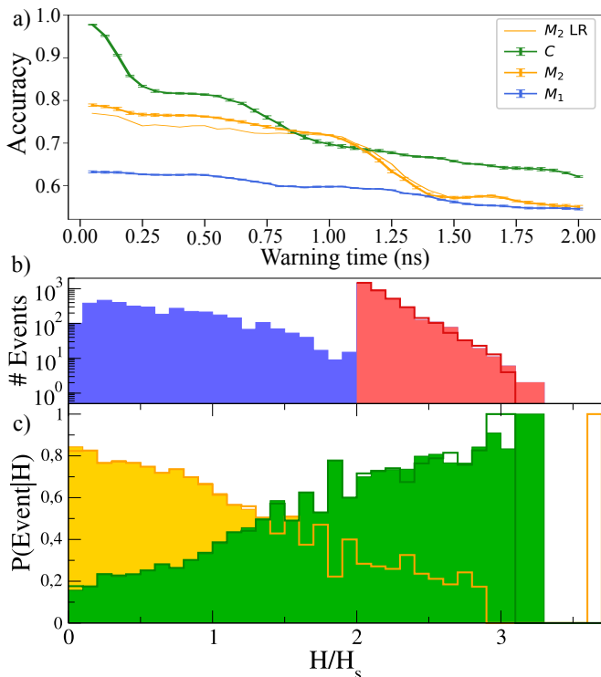
Figure 4. a) Mean EE forecasting accuracy at C with \tau_h = 1.75 ns versus the warning time, using either local (at C ) or nonlocal (at M_1 or M_2 ) data as input. The mean and standard deviation are computed with 10 different realizations of the reservoir. Thin line: nonlocal forecasting at M_2 using logistic regression alone. b) Histogram of the testing dataset heights distribution (blue, NE and red, EE events). c) classification probability as an EE (green) or a NE (complementary, orange) of an event of actual height H occurring \tau_w = 1 ns in the future at C from the knowledge of a history of \tau_h = 1.75 ns duration of the non-local data at M_2 . Two different realizations of the testing dataset are illustrated (plain and empty histograms).
