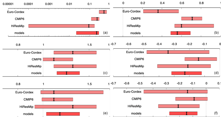
Figure 9. Projected changes between the present and +2°C climate. Summary of results for probability ratio ( a, c, e ) and change in intensity [°C] ( b, d, f ) in the three indices TNNApr–Jul ( a, b ), TNNGDD250 ( c, d ) and TNNGDD250–350 ( e, f ). Extent of the bars gives two-sided 95 % confidence intervals accounting for variability within the datasets, with the black marker indicating the best estimate. A weighted average of the results is shown in bright red.
