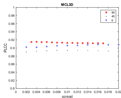
Fig. 5. PLCC of the DoC-GRNN scores for different directions of an array of line-shaped structuring elements used in the DoC-based decomposition.
