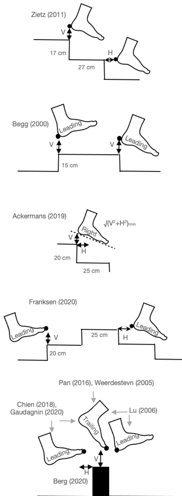
Figure 3: Foot clearance definitions from different studies. V, vertical; H, horizontal.
