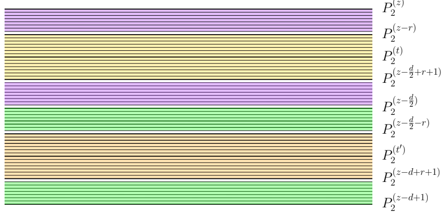
Figure 8: Visualization of the layers of W_2 that are subsets of \text{ann}(\mathcal{A}_z^{(d)}(W_2)) . For every h \in [\rho] , P_h := \text{Perim}(W^{2h+1}) . The color-shadowed areas follow the colors in Figure 2.
