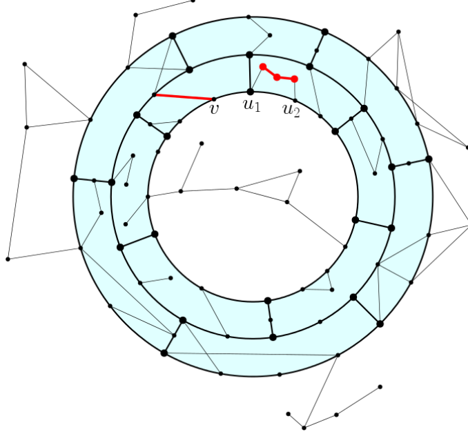
Figure 6: An example of an annulus-boundaried graph (G, K, Y, \mathbb{A}) . The annulus A is depicted in blue. Two wall-components of (G, K, Y, \mathbb{A}) are depicted in red: An edge attached to v \in V(G) and a subgraph of K attached to u_1, u_2 \in V(G) .
