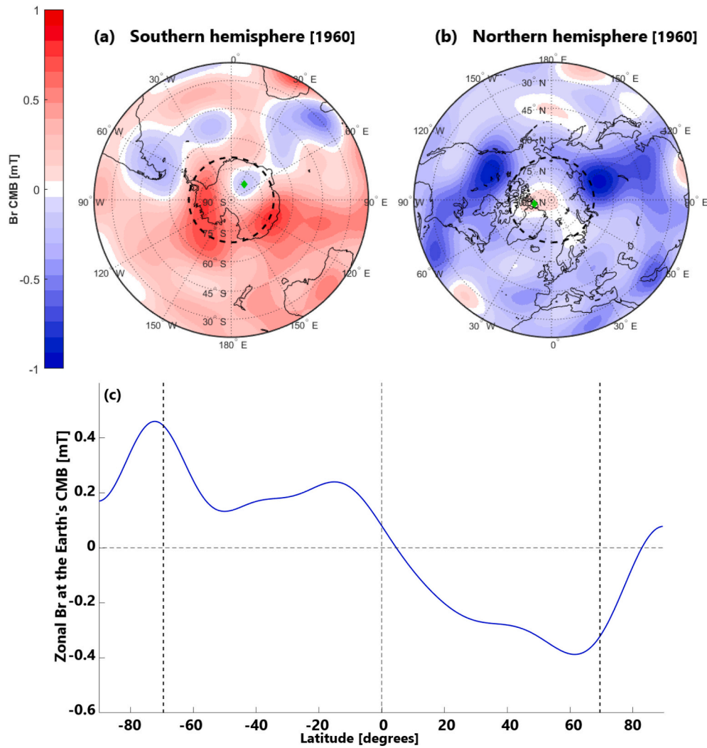
Fig. A1. As in Fig. 3 for the year 1960. Polar minima values for the northern hemisphere are \frac{|dB_r^z|}{\max|B_r^z|} = 1.01 ; \frac{|dB_r|}{\max|B_r^z|} = 2.25 ; \frac{S_{TC}^{sev}}{S_{TC}} = 23.25\% ; \lambda_{mean} = 82.78^\circ ; \lambda_{cm} = 81.69^\circ ; \phi_{cm} = -76.17^\circ . For the southern hemisphere \frac{|dB_r^z|}{\max|B_r^z|} = 0.63 ; \frac{|dB_r|}{\max|B_r^z|} = 1.36 ; \frac{S_{TC}^{sev}}{S_{TC}} = 13.45\% ; \lambda_{mean} = -80.17^\circ ; \lambda_{cm} = -80.19^\circ ; \phi_{cm} = 40.67^\circ .
