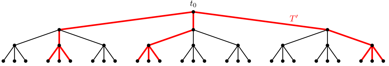
Figure 3: A rooted tree (T, t_0) and a \varphi -spanning subtree T' of T (depicted in red), for a sentence \varphi = \forall x_1 \exists x_2 \forall x_3 \psi(x_1, x_2, x_3) .
