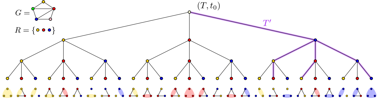
Figure 1: An example of an assignment of an annotated graph (G, R) (depicted on the upper left part of the figure) to a rooted tree (T, t_0) (in the center of the figure). We use colors for each vertex of G in order to distinguish them, without using indices and we use colors in the nodes of T to show where each vertex of G is mapped to. The small graphs below each leaf of T encode the pattern-coloring, i.e., are the (boundaried) graphs induced by the vertices collected in each root-to-leaf path of T and the linear orderings of their vertex sets (from left to right) follow the ordering of the corresponding path. Vertices that are picked twice in the same path are drawn inside a same-colored bag (respecting the ordering). The subtree T' is a \varphi -spanning subtree of (T, t_0) for the FOL-sentence \varphi = \exists x_1 \in R \forall x_2 \in R \exists x_3 \in R (x_1 = x_2 \vee E(x_2, x_3)) , that certifies that (G, R) \models \varphi .
