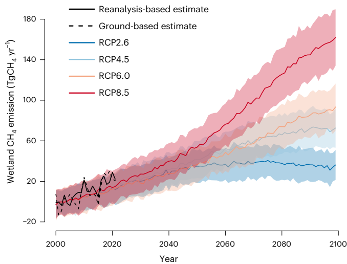
Fig. 1 | Temporal trends and variations in wetland CH 4 emissions during 2000–2021 relative to the baseline of 2000–2006 level in comparison to future projections 12 . Shaded areas present 1σ range of the estimates from each future RCP. Annual total emissions from two estimates based on two climate forcing datasets, a ground-based dataset from the CRU at the University of East Anglia and a reanalysis-based MERRA2. Coloured lines represent ensemble mean of each future projection scenario.
