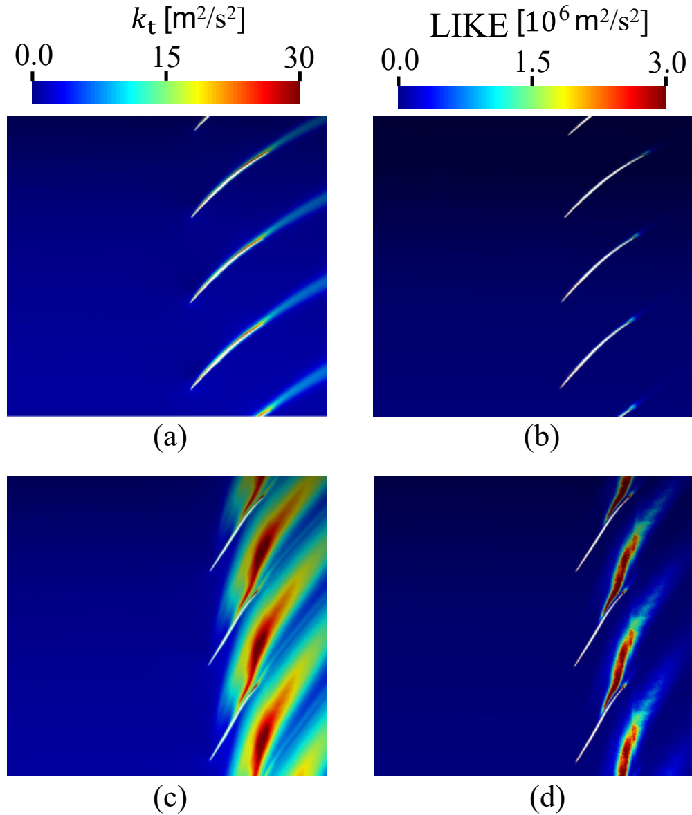
FIG. 12: Contours of (a,c) turbulent kinetic energy, (b,d) loss in turbulent kinetic energy 36 , around the rotor blade, at two spanwise positions, (a,b) 80%, (c,d) 99%.
