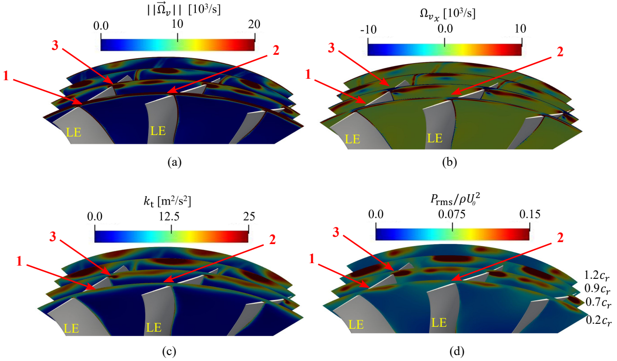
FIG. 15: Contours of averaged (a) vorticity magnitude, (b) axial vorticity component, (c) turbulent kinetic energy and (d) RMS pressure fluctuations at four different axial cross-sections in the blade passage. "LE" refers to the leading edge.
