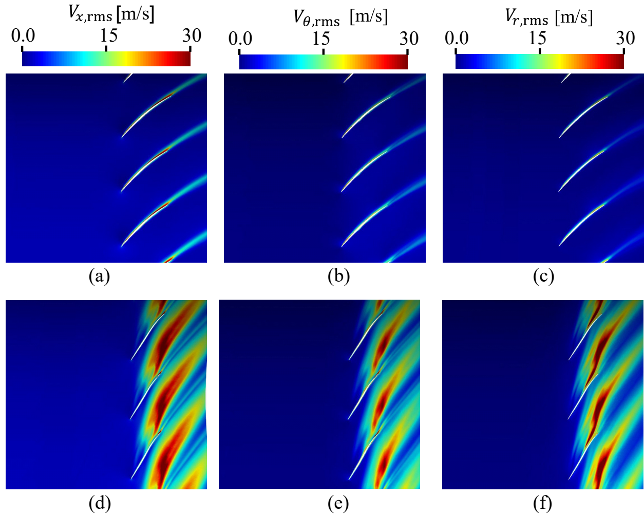
FIG. 10: Contours of the components of the RMS velocity fluctuations, around the rotor blade, at two spanwise positions, (a,b,c) 80%, (d,e,f) 99%.
