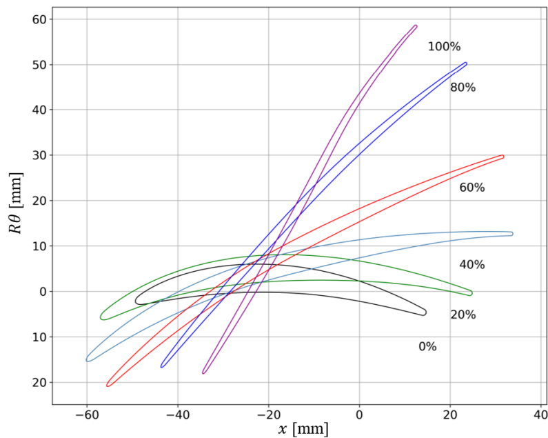
FIG. 3: Rotor profiles for different heights.
