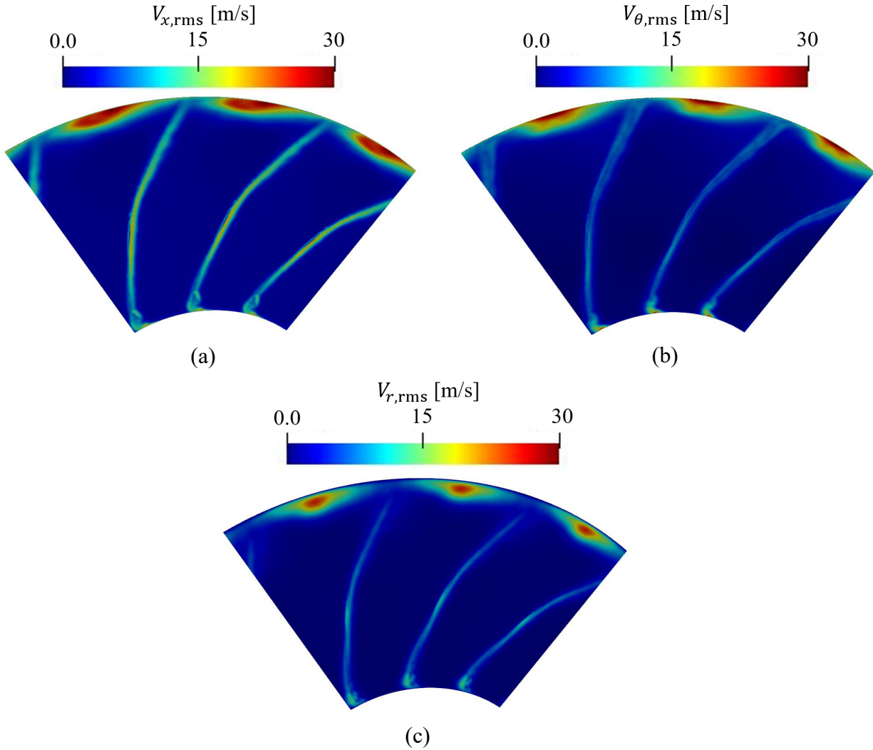
FIG. 11: Contours of the (a) axial, (b) circumferential and (c) radial components of the RMS velocity fluctuations on an axial plane directly downstream of the rotor trailing edge.
