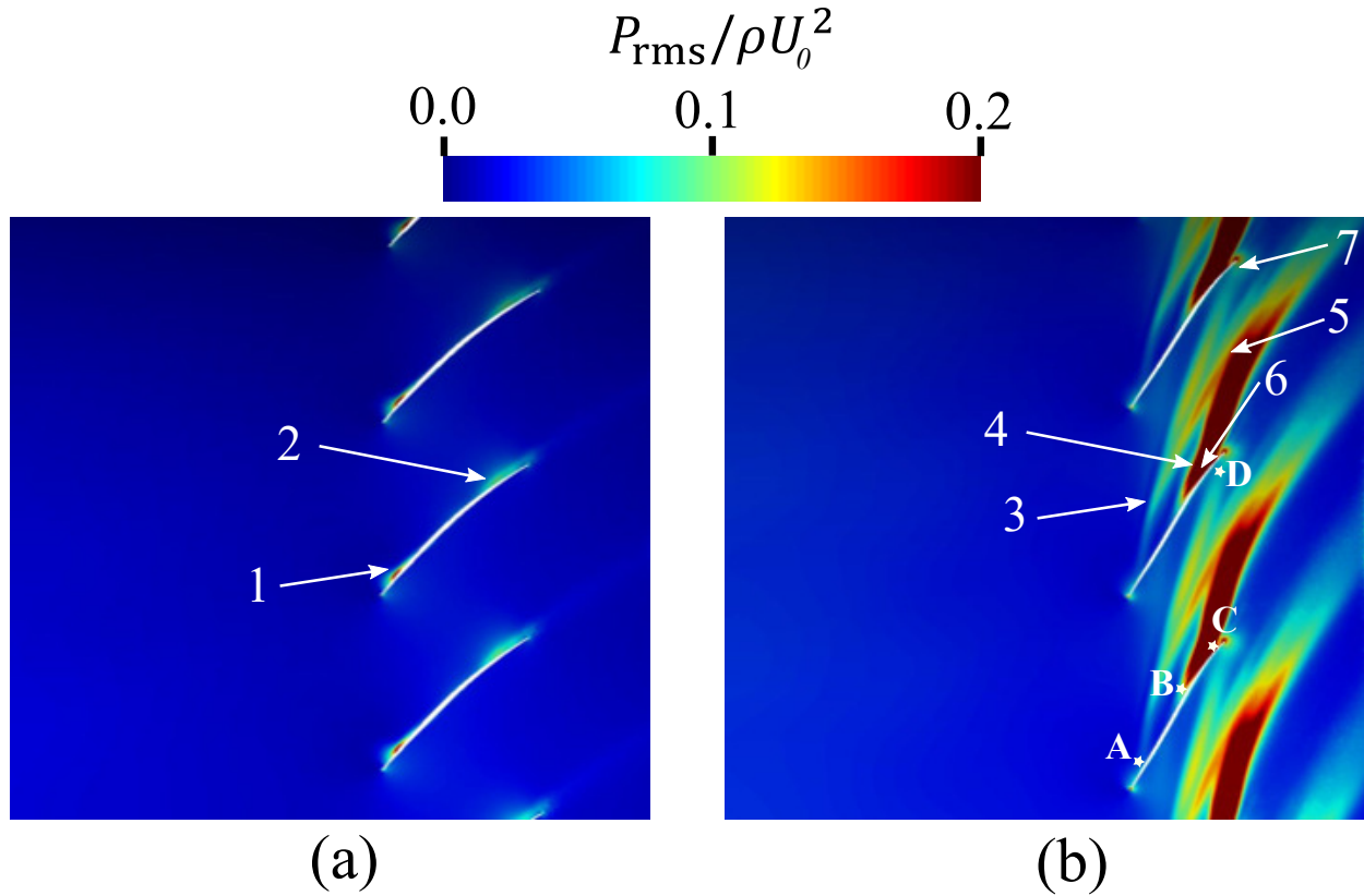
FIG. 13: Contours of RMS pressure fluctuations around the rotor blade, at two spanwise positions, (a) 80%, (b) 99%. The star symbols show the positions of the monitor points, "A", "B", "C" and "D", used for the computation of the coherence in the tip-gap region.
