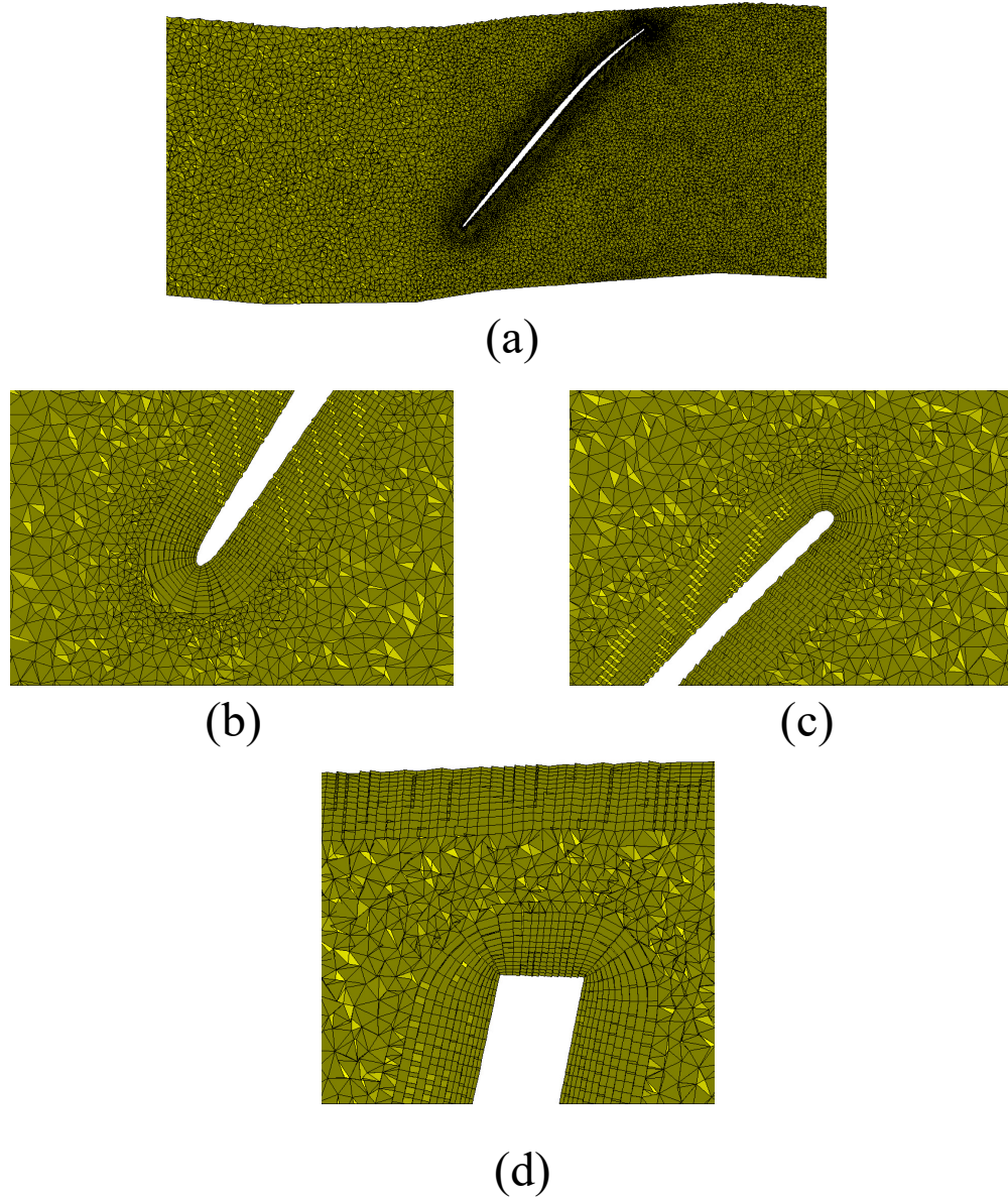
FIG. 4: (a) Mesh around the rotor blade at 95% of the span. Mesh refinements near the rotor leading edge (b), the rotor trailing edge and in the rotor tip-clearance region (d).
