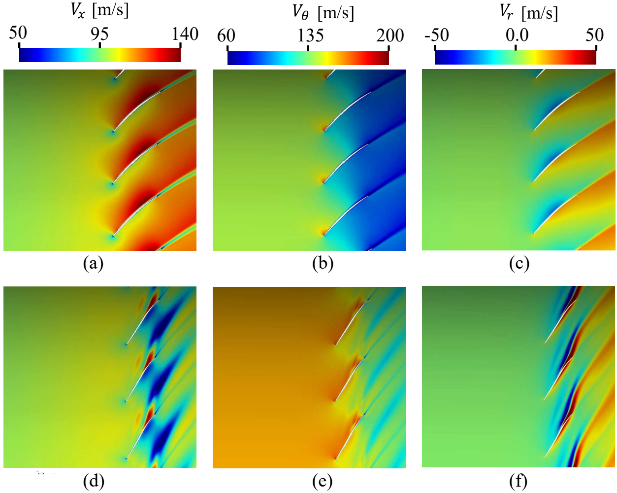
FIG. 9: Contours of the averaged velocity components around the rotor blades for two spanwise positions, (a,b,c) 80%, (d,e,f) 99%.
