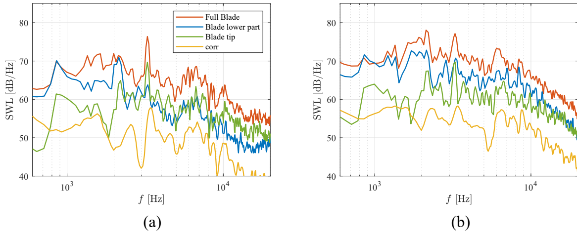
FIG. 24: SWL spectra from the FWH analogy 19 for the full blade (denoted "Full Blade"), the tip-gap region (denoted "Blade tip"), the lower part of the blade (denoted "Blade lower part") and the cross-correlation between them (denoted "corr"). (a) Upstream direction. (b) Downstream direction.
