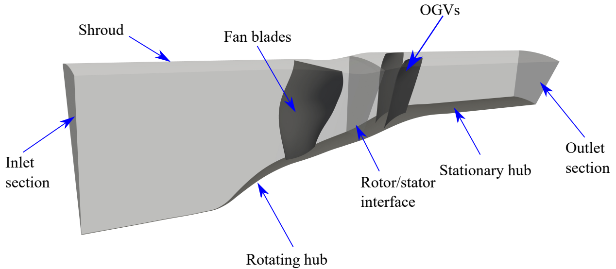
FIG. 2: Computational domain of the ECL5 fan/OGV stage.
