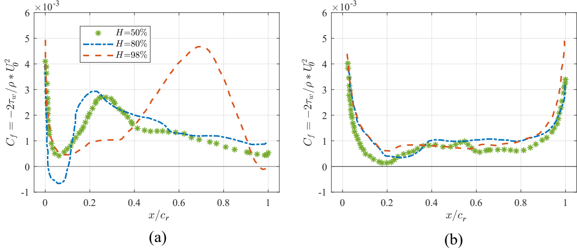
FIG. 16: Averaged friction coefficient, C_f , along the rotor blade at different spanwise positions.
