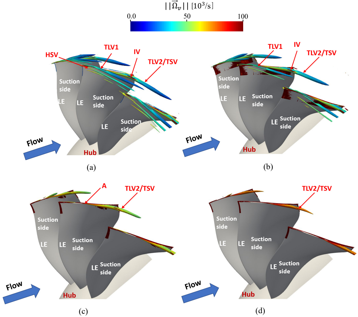
FIG. 8: Averaged Q-criterion in the tip-gap region, colored by the vorticity magnitude, for different iso-surface values, (a) \overline{Q}c_r^2/U_0^2 = 500 , (b) \overline{Q}c_r^2/U_0^2 = 750 , (c) \overline{Q}c_r^2/U_0^2 = 1000 , and (d) \overline{Q}c_r^2/U_0^2 = 1250 .
