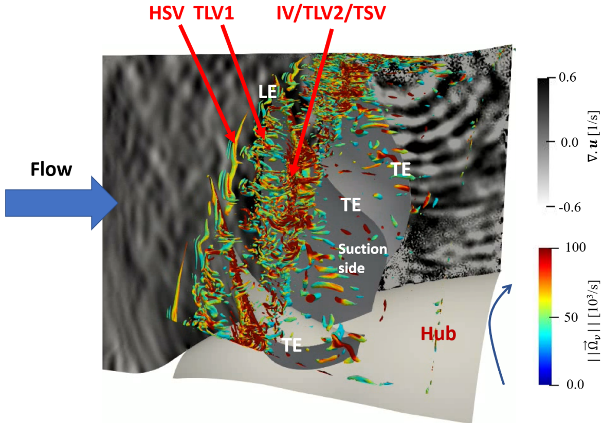
FIG. 17: Instantaneous contours of dilatation rate in a cross-section that intersects the rotor blade, and iso-surfaces of Q-criterion ( Qc_r^2/U_0^2 = 100 ) colored by the vorticity magnitude in the tip-gap region. "LE" refers to the leading edge and "TE" refers to the trailing edge.
