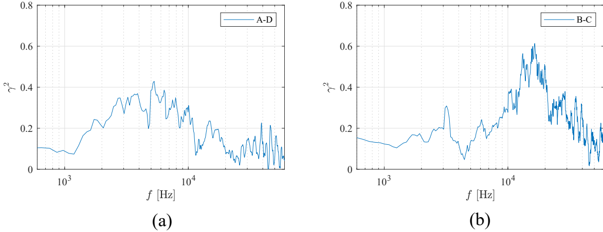
FIG. 22: Coherence between the pressure fluctuations at the monitor points "A" and "D" (a), and the monitor points "B" and "C" (b).
