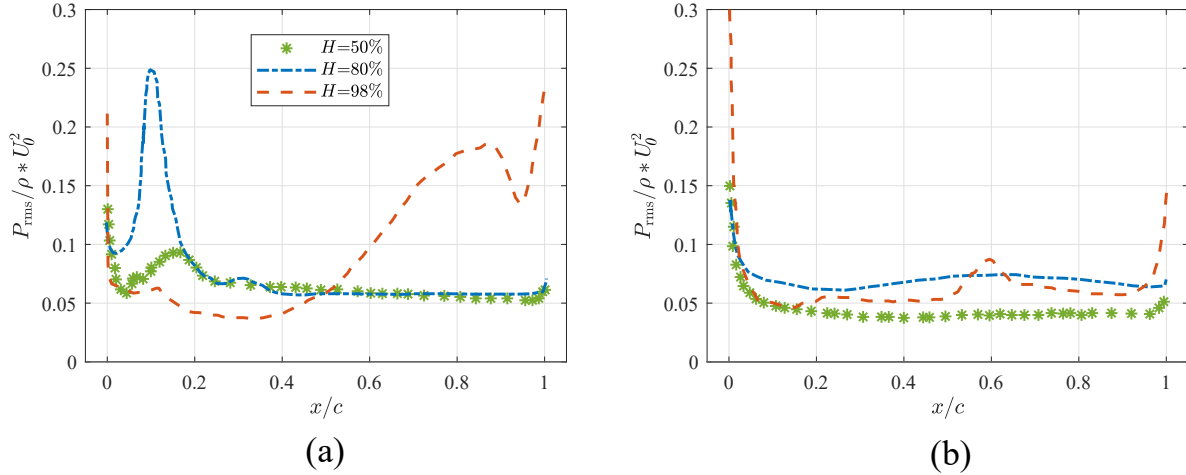
FIG. 19: RMS pressure fluctuations P_{\text{rms}} along the rotor blade, at different spanwise positions. (a) Suction side. (b) Pressure side.
