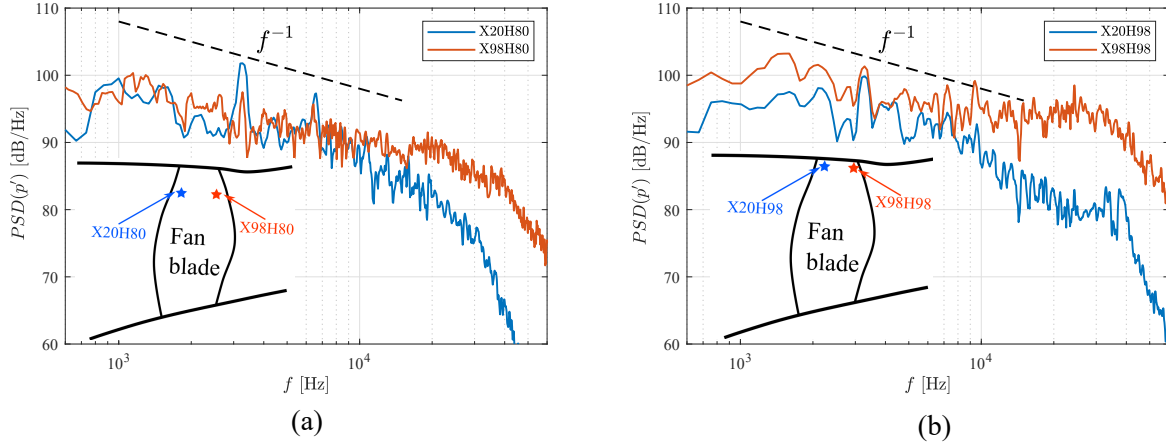
FIG. 20: WPS on the suction surface of the rotor blade, at several positions (a) 80% and (b) 98% of the rotor span. p' corresponds to the pressure fluctuation. The reference pressure is
