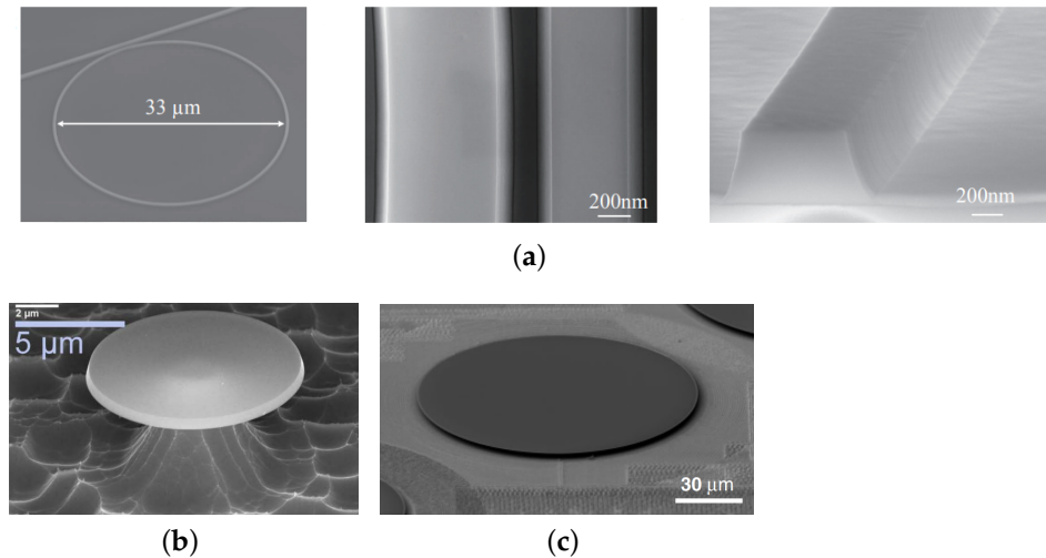
Figure 3. Scanning electron microscope images of (a) 4H SiCOI MMR, reprinted with permission from [36] ©The Optical Society, (b) 3C SiC MDR [59], and (c) 4H SiCOI MDR [56].
