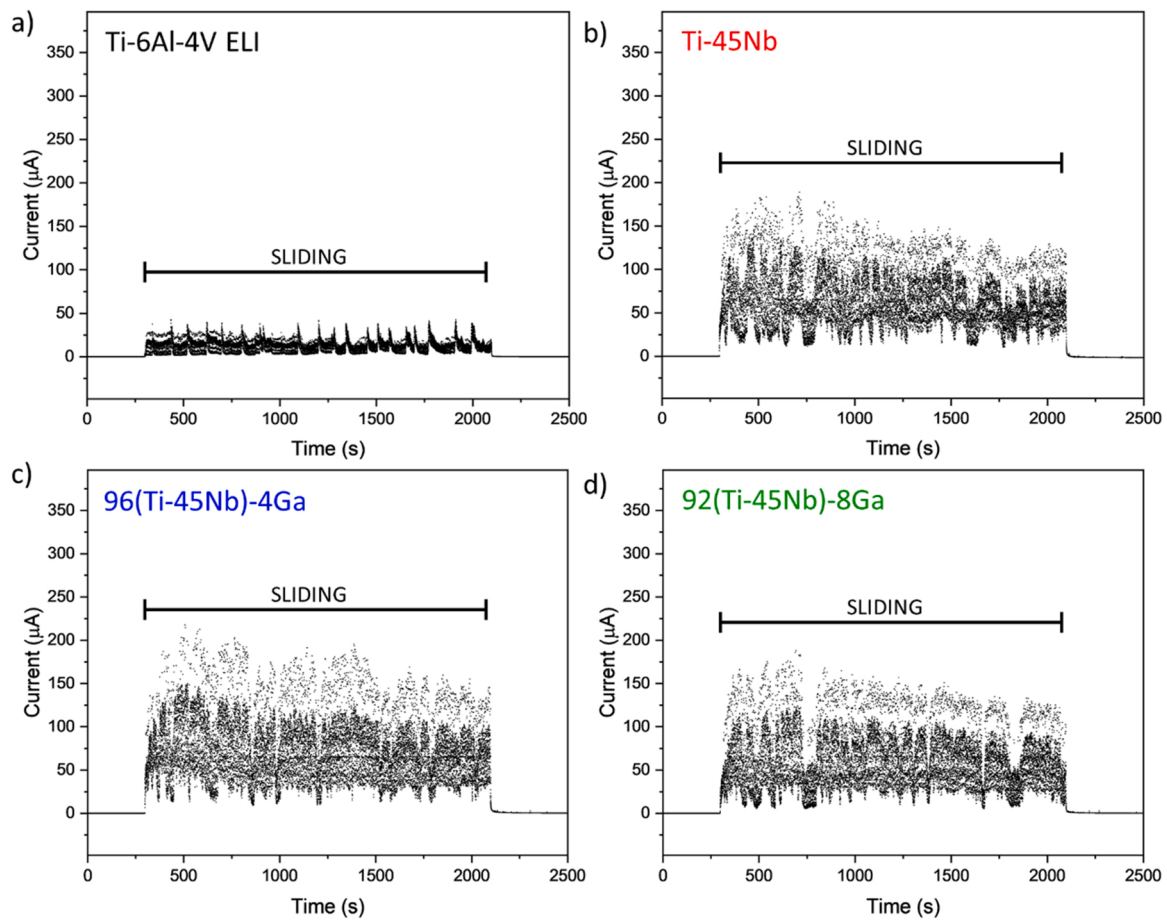
Fig. 5. Current evolution with time during sliding (load 5 N) with an alumina pin against (a) Ti-6Al-4V ELI, (b) Ti-45Nb, (c) 96(Ti-45Nb)-4Ga, (d) 92(Ti-45Nb)-8Ga at applied potential (0 V vs final OCP) in PBS solution.
