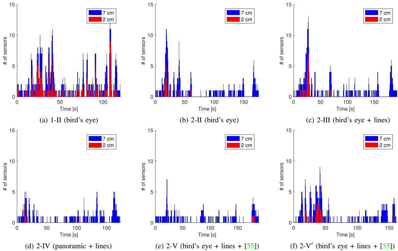
Fig. 9: First experimental campaign . Number of sensors which detected an obstacle at a distance of less than 7 cm (blue) or 2 cm (red). The Arabic (Roman) numerals in the captions under each plot, refer to the subjects (trials).
