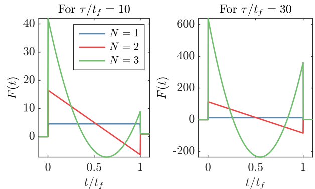
FIG. 1. Driving function F(t) to apply in order to cancel successively the first thermal modes for an acceleration (towards the stationary profile) such that t_f = \tau/10 (left) and t_f = \tau/30 (right). The coefficients \gamma_n defining F(t) are found solving Eq. (10); they are listed in table I of Appendix A.
