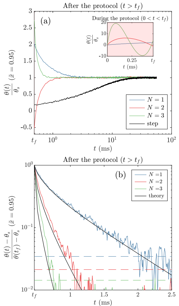
FIG. 7. (a) Temperature relaxation towards the stationary state (measured close to the cantilever free end \tilde{x} = 0.95 ) varying N for a protocol duration t_f = \tau/30 = 0.47 ms. Inset: temperature variations during the protocol. (b) Comparison of the temperature decay. The horizontal dashed lines correspond to a relative difference (\theta - \theta_s)/\theta_s of 4%.
