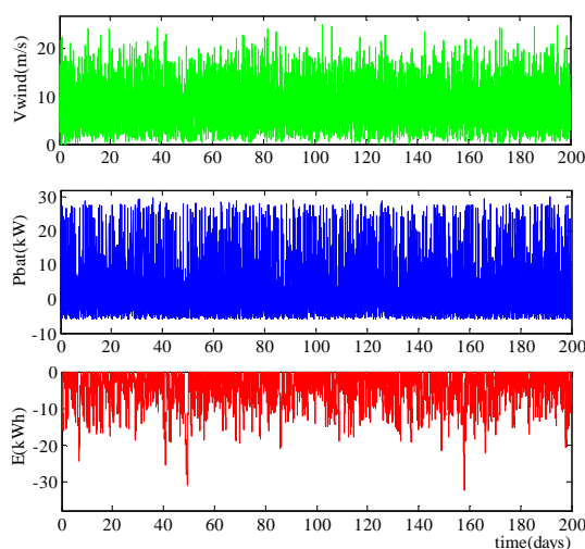
Figure 3. Actual 'reference' wind speed profile, storage power and energy.
