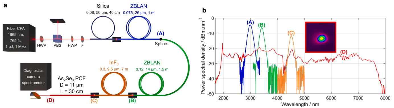
Fig. 1. (a) Schematic of the setup used for the generation of fiber-based two-octave spanning mid-IR SC. HWP: half-wave plate, PBS: polarization beam splitter, F: focusing lens. The fibers are characterized by their NA, core diameter and length. (b) Spectra measured at four positions in the cascaded fiber system. The inset shows the near-field intensity distribution measured at the output of the chalcogenide fiber.
