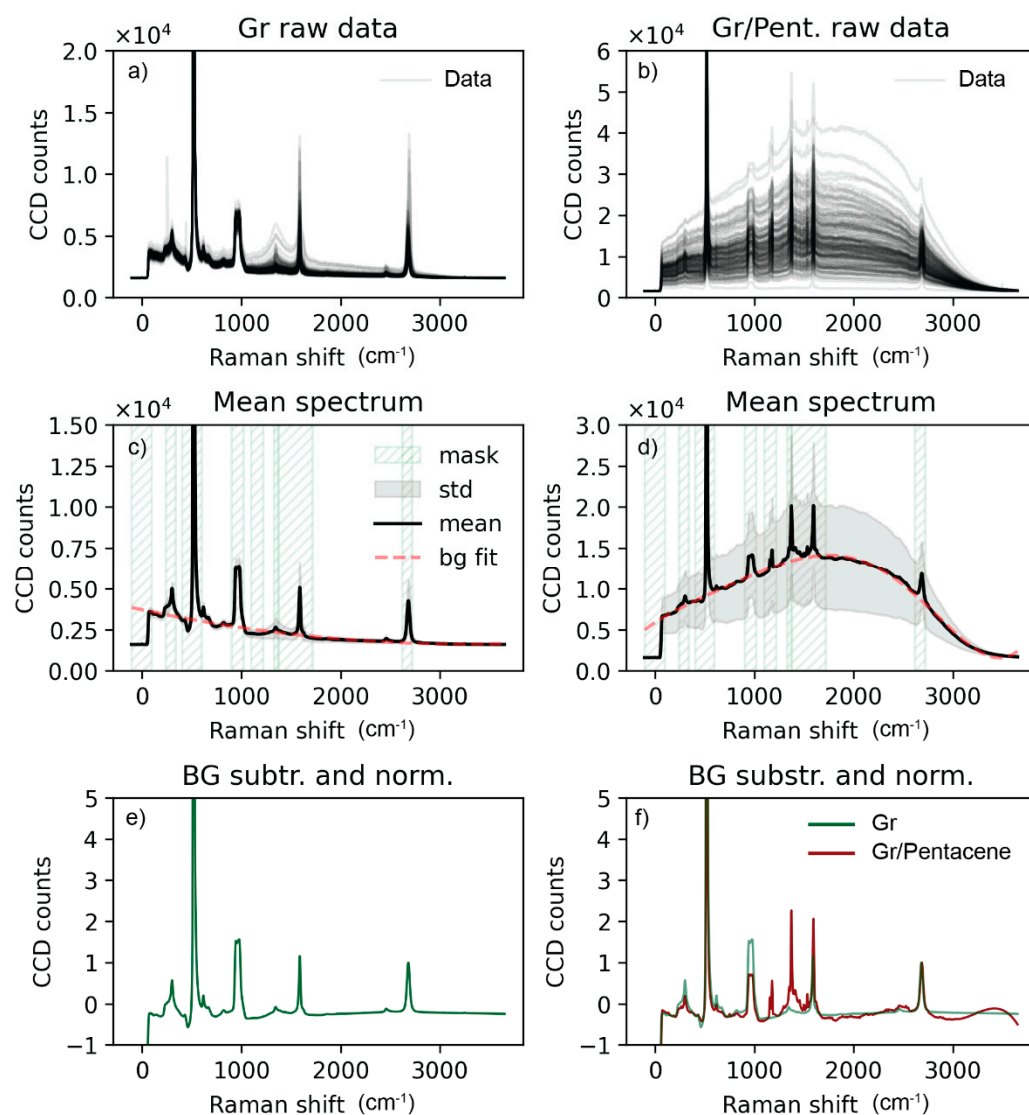
Figure S3. Raman spectrum of the Gr/Pentacene heterostructures. (a) Raman spectra of the 150 pristine CVD Gr channels. (b) Raman spectra of the 150 Gr/Pentacene channels. (c) Average Raman spectrum of the 150 measurements of the pristine CVD Gr in (a). The red dashed line is the polynomial fit (degree 2) of the background. The green hatched areas (mask) are not considered in the polynomial fit. (d) Average Raman spectrum of the 150 measurements of the Gr/Pentacene heterostructure in (b). The red dashed line is the polynomial fit (degree 5) of the background. The green hatched areas (mask) are not considered in the polynomial fit. (e) Pristine CVD graphene Raman spectrum after background removal and normalization to the 2D peak of graphene. (f) Raman spectrum of the Gr/Pentacene heterostructure after background removal and normalization to the 2D peak of graphene.
