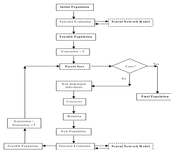
Figure 1. Scheme of Optimization Procedure
