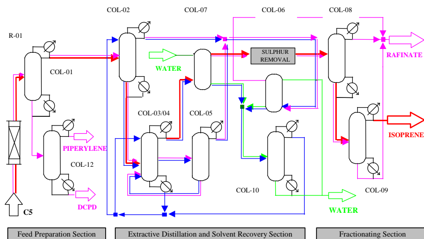
Figure 2. Isoprene Unit
