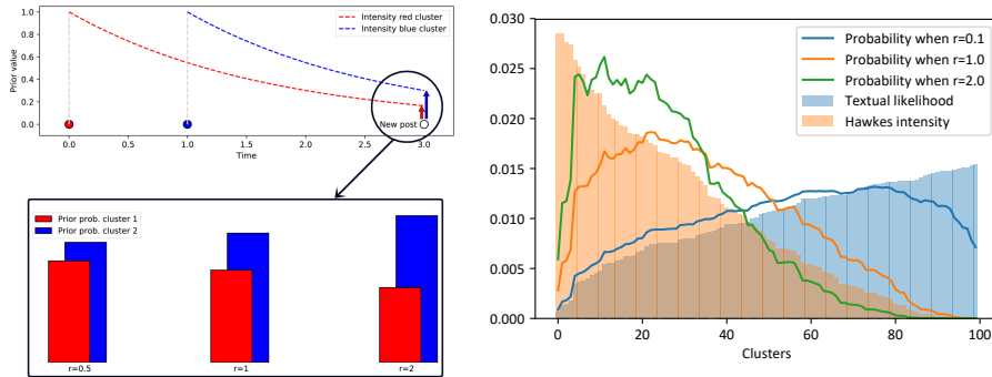
Fig. 2. Effect of r on cluster selection probabilities — The probability for each cluster to get chosen (solid lines) for several values of r and fixed individual textual likelihood (blue bars) and Hawkes intensity (orange bars).
