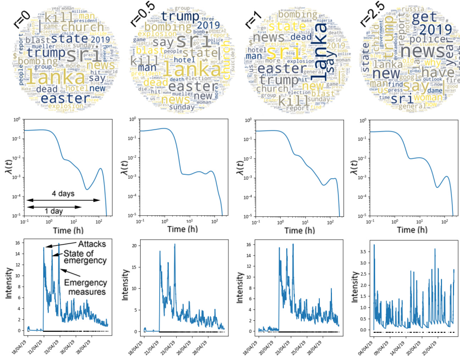
Fig. 9. Wordclouds, triggering kernels and intensities for clusters the most closely related to Sri Lanka 2019 bombings for various values of r . The points at the bottom of the intensity plots are individual publication events. Note that triggering kernels are plot on a log-log scale for visualisation purpose, because most of the intensity is focused on small times: dynamics are bursty.
