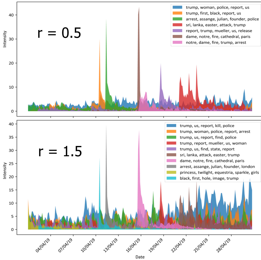
Fig. 12. PDHP allows for modeling bursty events — We plot PDHP’s intensity for the News dataset over the observation period for two values of r . The clusters plot here are the ones out of \sim 300 clusters that have an intensity going above 10 at least once. A lower r finds globally relevant clusters, whereas a higher r allows to recover shorter bursty events.
