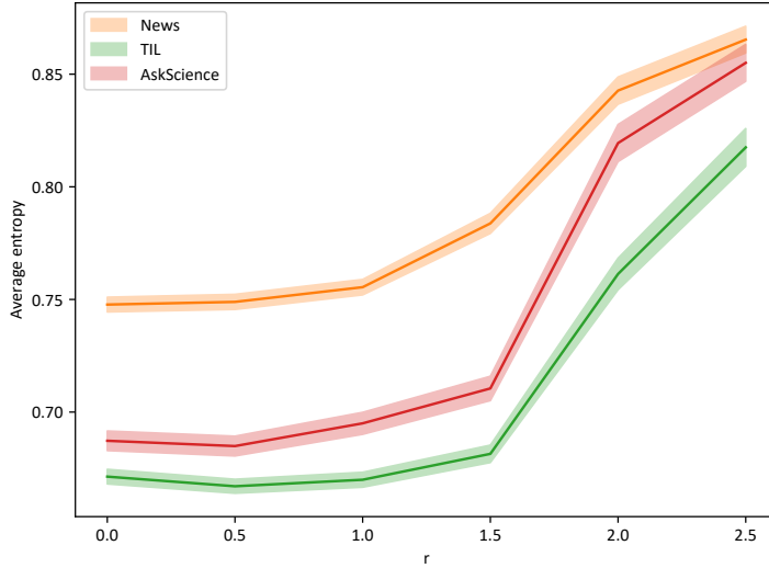
Fig. 11. Textual clusters are more informative for low values of r — Weighted average entropy of words distribution for every dataset. Weights corresponds to the number of words within clusters. The error bar represents the standard error over all the clusters.
