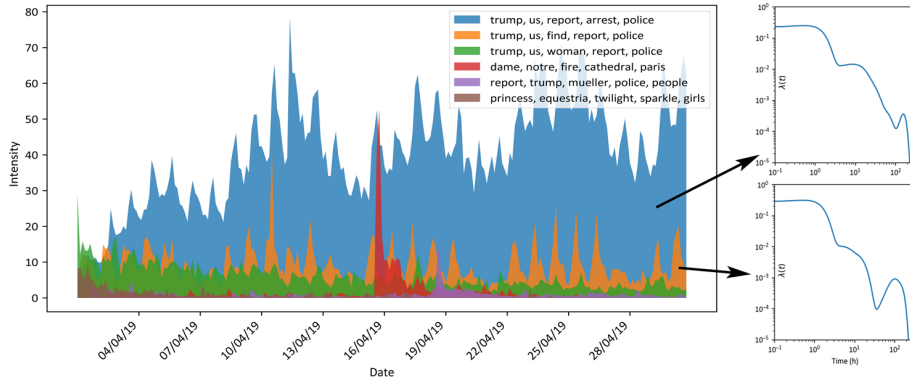
Fig. 13. Limit case of encouraging bursty events clustering — We plot PDHP’s intensity for the News dataset over the observation period for a large value of r . In this case, textual information plays a marginal role, and clusters are inferred based on the events publication dates only.
