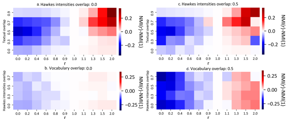
Fig. 5. PDHP performs better than DHP — Difference between the normalized mutual information (NMI) of PDHP and DHP model (Du et al., 2015) for various values of r , intensities overlap and vocabulary overlap, averaged over all the datasets. Red means PDHP performed better, blue means PDHP performed less well. Because \text{PDHP}(r = 1) = \text{DHP} , the column r = 1 show no difference. PDHP allows to increase results on NMI by as much as 0.3 over DHP.
