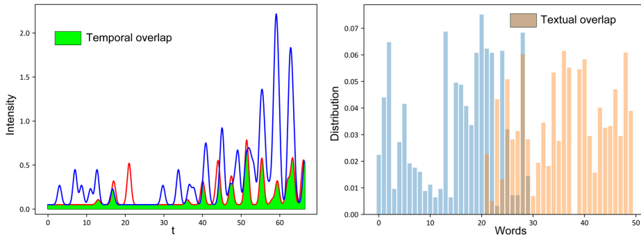
Fig. 3. Overlaps — (Left) Temporal overlap is defined as the ratio between the area common to two Hawkes intensities and the total area under the intensity functions. (Right) Textual overlap is defined as the proportion of vocabulary that is common to two clusters, weighted by the probability of words within their respective cluster.
