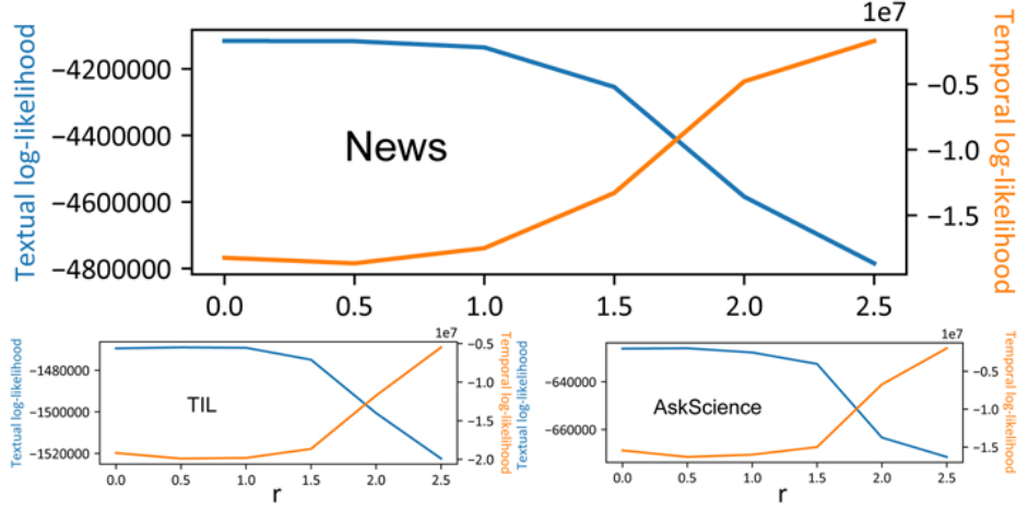
Fig. 10. r allows to favour text-based or time-based clustering on real world datasets — Textual likelihood and Hawkes process likelihood for various values of r . The lower r the higher textual likelihood is, and the higher r the higher Hawkes process likelihood is.
