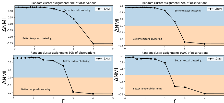
Fig. 7. Varying r allows to choose between textual or temporal clustering — The black line plots the difference between the NMI of textual and temporal clustering. For small r , textual clustering is far better than temporal clustering, and for large r , the situation is reversed. This is because r determines the importance given to the temporal dimension and therefore allows choosing between retrieving temporal or textual clusters.
