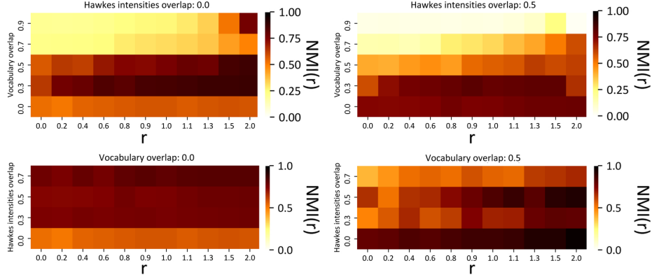
Fig. 4. PDHP yields good NMI values — Normalized mutual information (NMI) for various values of r , intensities overlap and vocabulary overlap, for one dataset per combination. The results for r = 0 are the output of the Uniform process, the results for r = 1 are the output of the DHP (Du et al., 2015), and the other values of r correspond to other special cases of PDHP. The darker the better. Overall, PDHP yields good values of NMI.
