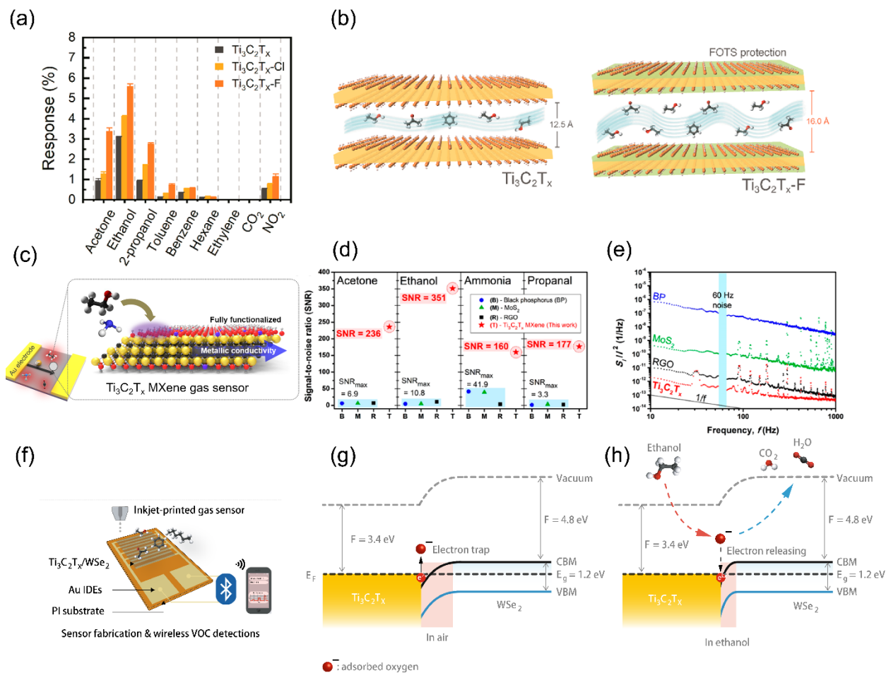
Fig. 17. VOC sensing examples of MXene-based chemiresistors. (a) Maximal response changes upon exposure to various gases. (b) Schematics of \text{Ti}_3\text{C}_2\text{T}_x and \text{Ti}_3\text{C}_2\text{T}_x\text{-F} upon exposure to VOCs. FOTS passivation of \text{Ti}_3\text{C}_2\text{T}_x MXene prevents it from oxidation, enabling a longer shelf-life. Reprinted with permission from ref. 390 . Copyright 2020 American Chemical Society. (c) Schematic illustration of the \text{Ti}_3\text{C}_2\text{T}_x films and its atomic structure. (d) Maximal SNR values of sensors upon exposure to 100 ppm of acetone, ethanol, ammonia, and propanal. (e) Flicker noise measured by normalized noise power spectral density ( S_I/I^2 ) as a function of frequency. Reprinted with permission from ref. 391 . Copyright 2018 American Chemical Society. (f) Schematic illustration of inkjet-printed gas sensors based on \text{Ti}_3\text{C}_2\text{T}_x/\text{WSe}_2 in detection of volatile organic compounds with a wireless monitoring system. Enhanced sensing mechanism of \text{Ti}_3\text{C}_2\text{T}_x/\text{WSe}_2 heterostructure. Energy-band diagram of the \text{Ti}_3\text{C}_2\text{T}_x/\text{WSe}_2 in (g) air and (h) ethanol, showing the variation of the depletion layer with interaction between adsorbed oxygen species and ethanol molecules. Reprinted with permission from ref. 392 . Copyright 2020 Nature.
