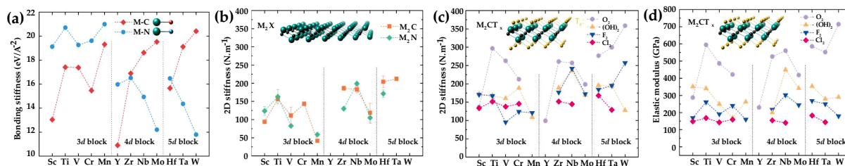
Fig. 2. (a) the bonding stiffness values for early transition metals, (b) the 2D stiffness of pristine MXenes, (c) the 2D stiffness of the terminated MXenes (d) the elastic modulus of the terminated MXenes. Adapted from Ref. 88 . Copyright © 2021.
