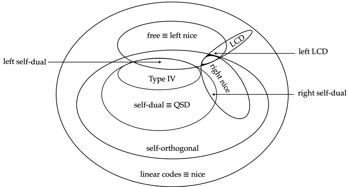
Figure 2: Classes of linear codes over the ring E
