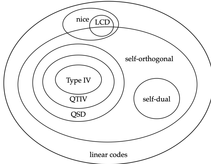
Figure 3: Classes of linear codes over the ring H
