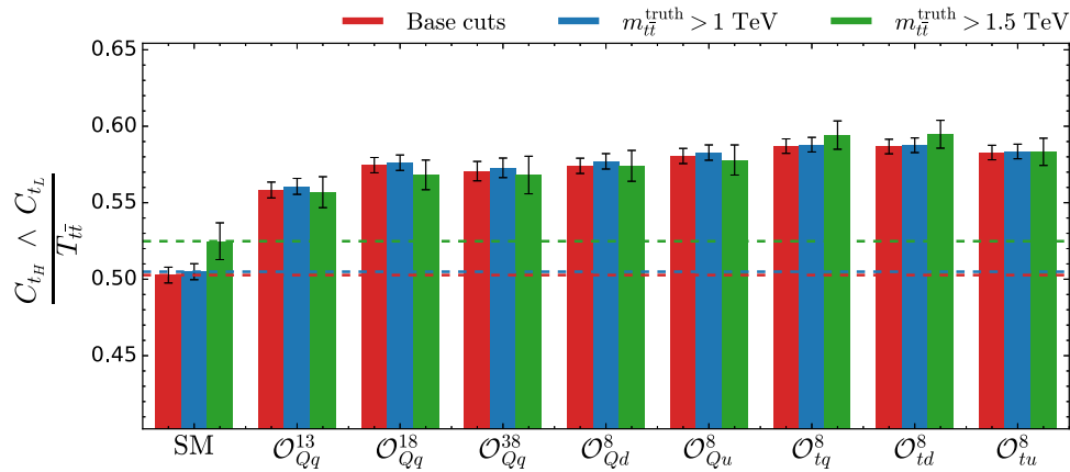
Fig. 2 Efficiency associated with the reconstruction of one leptonic top quark and one hadronic top quark, estimated relatively to the number of events containing two on-shell top quarks. Results are shown after the analysis baseline cuts (red), an additional m_{t\bar{t}}^{\text{truth}} > 1 TeV cut (blue), and an extra m_{t\bar{t}}^{\text{truth}} > 1.5 TeV cut (green). We consider the case of the SM (first column), as well as when eight different SMEFT operators are turned on (next columns)
