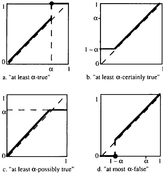
Fig. 1. Four basic types of fuzzy truth-values
