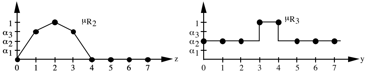
Figures 3a and 3b. Modeling of C_2 (a) and C_3 (b) by means of fuzzy unary restrictions
