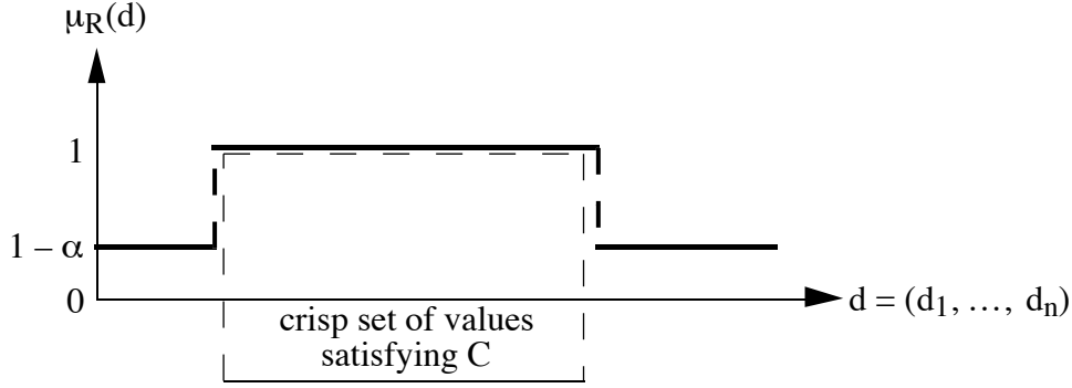
Figure 1. A hard (or crisp) constraint C with priority \text{Pr}(C) = \alpha when c(x) = 1 - x .
