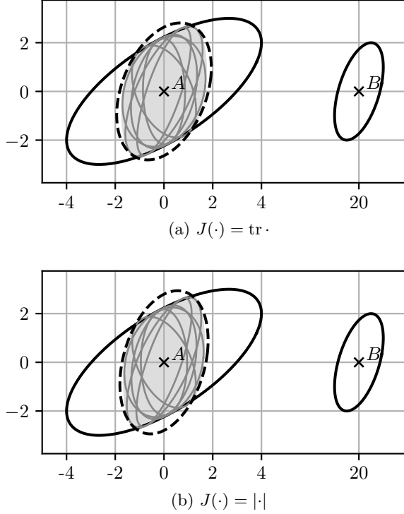
Figure 1: Example of the optimal SCI filters for two different cost functions J . The black solid ellipses represent the covariance of the estimators \mathbf{P}_A and \mathbf{P}_B . The dashed ellipse represents the covariance of the optimal SCI filter \mathbf{P}_{\text{SCI}}^* . The grey solid ellipses represent possible covariances \tilde{\mathbf{P}}_F obtained by (7) with \underline{w}_F = \underline{w}_{\text{SCI}}(\omega^*) and different \tilde{\mathbf{P}} \in \mathcal{P} , and the grey area their convex hull. In both figures: \mathbf{P}_A = [16, 8; 8, 9] , \mathbf{P}_B = [1, 1; 1, 4] , and \sigma_m^2 = 1 . The optimal parameters are \omega^* \approx 0.28 for the trace and \omega^* \approx 0.36 for the determinant.
