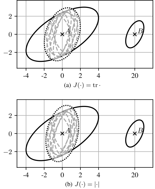
Fig. 1: Example of the optimal SCI filters for two different cost functions J . The solid ellipses represent the covariance of the estimators \mathbf{P}_A and \mathbf{P}_B . The dotted ellipse represents the covariance of the optimal SCI filter \mathbf{P}_{\text{SCI}}^* . The dashed ellipses represent possible covariances \tilde{\mathbf{P}}_F obtained by (7) with \underline{w}_F = \underline{w}_{\text{SCI}}(\omega^*) and different \tilde{\mathbf{P}} \in \mathcal{P} . The measurement variance is \sigma_m^2 = 1 .
