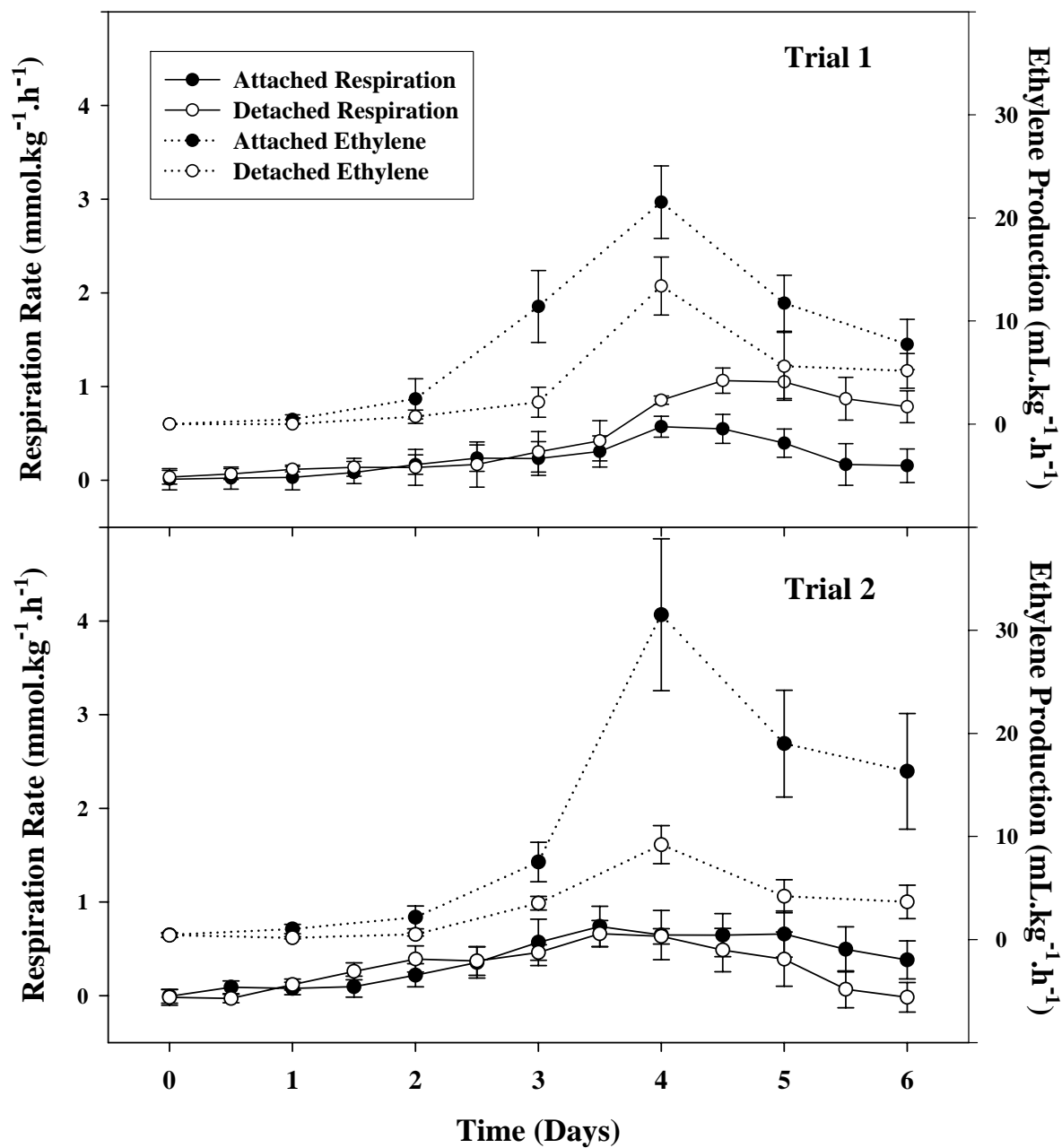
Fig. 1. Respiration rates and ethylene production of Charentais melons during ripening either attached to the vine or removed from the plant. The plants were grown at Toulouse, France (Trial 1) and Richmond, Australia (Trial 2). Each data point represents the mean of three fruit and the error bars are the standard errors of the means.
