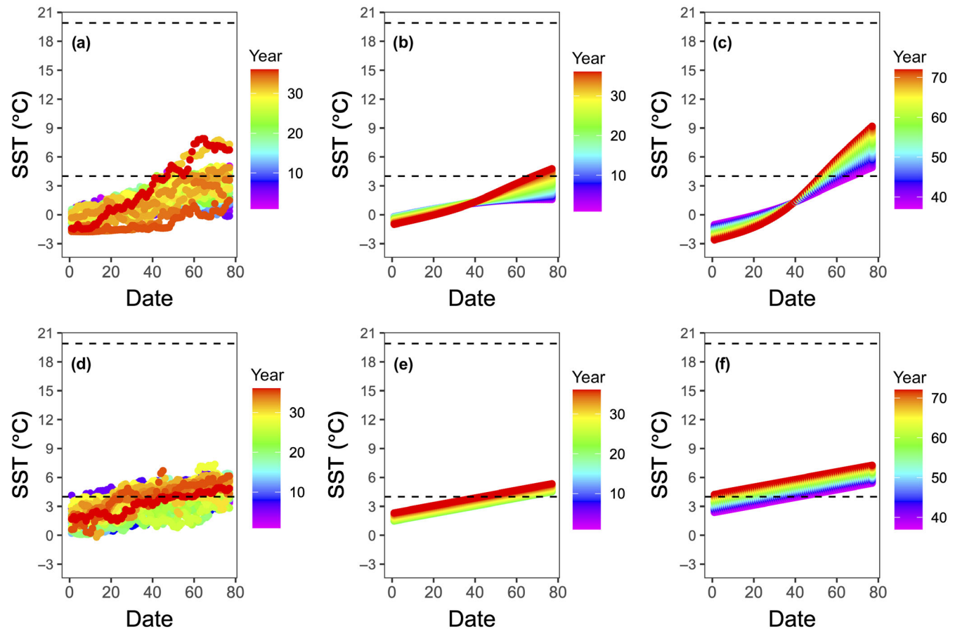
FIGURE 3 Temporal trends in sea surface temperature (SST) between June 1 (day 0) and August 15 (day 76), at Ukaleqarteq (UK) (a–c) and Horsund (HS) (d–f). Observed SST at (a) UK and (d) HS are shown between 1986 (Year 1) and 2021 (Year 36), along with predicted values from generalized additive models (GAMs) between 1986 and 2021 ([b] UK and [e] HS), and predicted values from GAMs projecting SST 36 years into the future, until 2057 (Year 72) ([c] UK [f] HS). The lower horizontal dashed line indicates 4°C, and the higher line 19.9°C, the temperatures at which daily energy expenditure is projected to surpass \sim 4 \times BMR and \sim 7 \times BMR.
