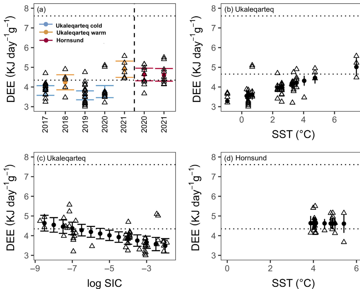
FIGURE 1 Variation in mass-specific DEE with (a) site-year, color coded with respect to average annual SST at UK (warm years >2.5^{\circ}\text{C} ; cold years <2.5^{\circ}\text{C} ), and with a distinct color for HS, (b) SST at UK, (c) SIC at UK and (d) SST at HS. Bars show 95% CIs around predicted values. Open triangles are observed values for individuals, with average SST/SIC and DEE calculated across accelerometer deployment periods. The vertical dashed line in (a) divides the sites. Dotted horizontal lines denote postulated DEE thresholds of \sim 4 and 7 \times \text{BMR} . BMR, basal metabolic rate; DEE, daily energy expenditure; HS, Hornsund; SIC, sea ice coverage; SST, sea surface temperature; UK, Ukaleqarteq.
