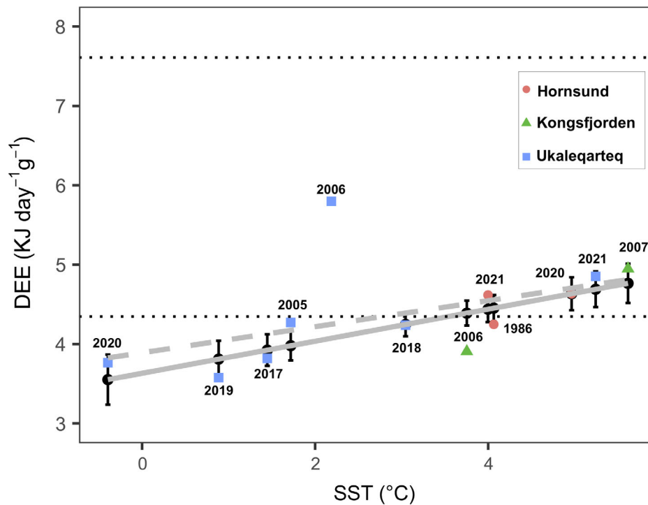
FIGURE 2 Relationship between average DEE of little auks and SST across 12 site-year observations from 1986 to 2021 at three sites. This relationship was non-significant when retaining the outlier (dashed line), but significant when removing this point (solid line). 95% CIs around predicted values are shown with the outlier removed. Points show experimental observations color-coded by study site. Observation year is indicated adjacent to each point. Dotted horizontal lines denote postulated DEE thresholds of \sim 4 and 7 \times BMR. BMR, basal metabolic rate; DEE, daily energy expenditure; SST, sea surface temperature.
