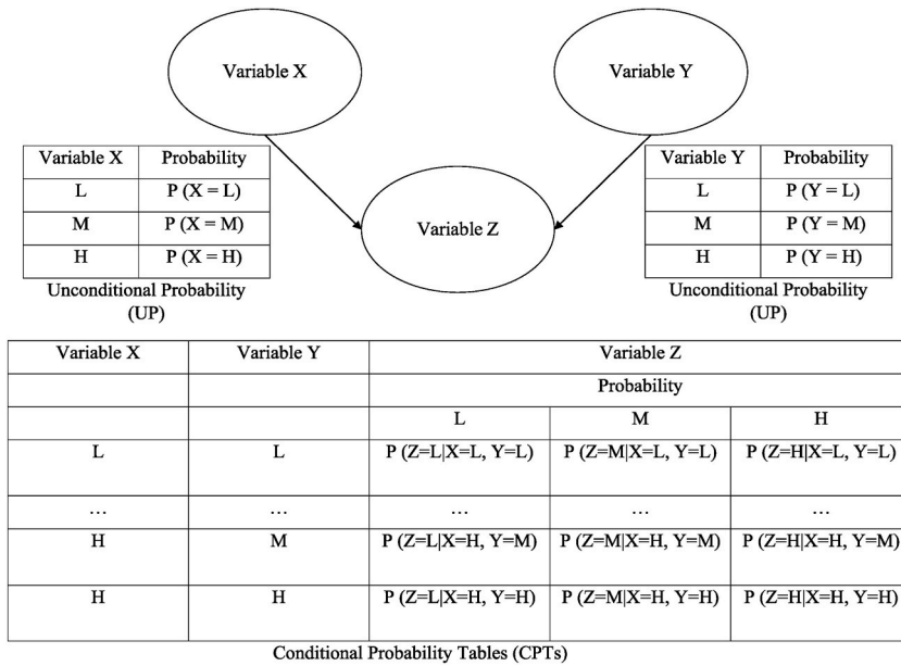
Fig. 9. Architecture of Bayesian networks.
