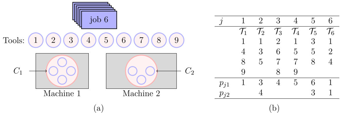
FIG. 1: A schematic layout example of the problem environment.
