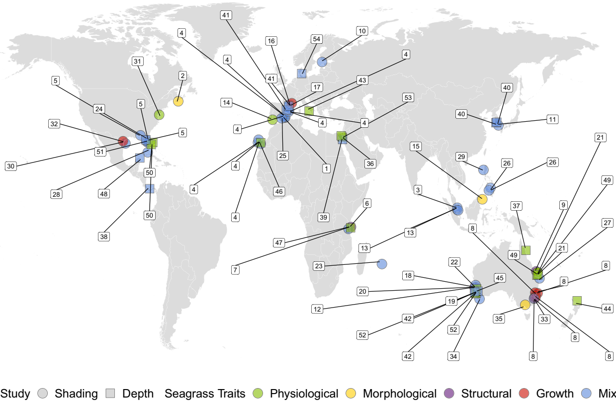
FIGURE 1 Results of the literature review. Shape shows the type of study (manipulative shading and depth-based studies) and colour the type of trait (physiological, morphological, structural and growth) studied in each publication (54 publications and 78 studies). The numbers related to each point represent the ID number corresponding to each publication in the Supporting Information (Table S1 in Appendix S1).
