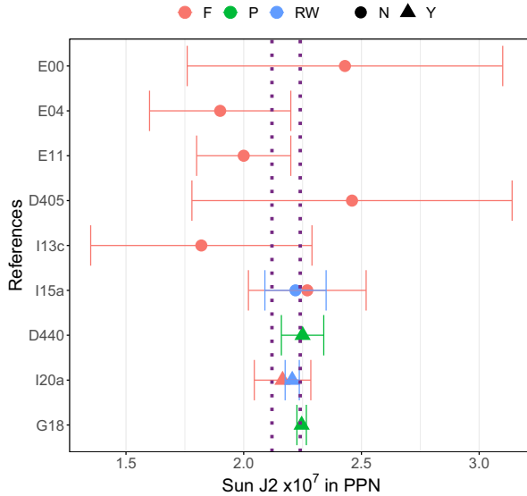
Fig. 9 Values of the Sun oblateness J_2^\odot obtained when considering PPN parameters \beta and \gamma as varying parameters. The dotted lines give the limits of the less constraining helioseismologic value from Pijpers (1998). F stands for Full fit, RW for random walk exploration method and P for partially fitted ephemerides (some parameters are fixed). N (respectively Y) indicates that the value has been obtained without (respectively with) LT. In y-axis, are given the references: G18 is Genova et al. (2018), I20a (Fienga et al. 2021a), D440 (Park et al. 2017), I13c (Fienga et al. 2014), E04 and E11 in Pitjeva and Pitjev (2013). E00 is Pitjeva (2001), D405 (Standish 2001) and I15a (Fienga et al. 2015). It is important to note that in Genova et al. (2018), only the orbit of Mercury is considered
