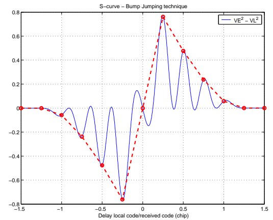
Figure 7: Bump-Jumping discriminator
