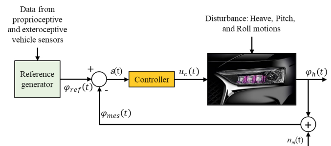
Fig. 6. Block diagram of the AHLS
