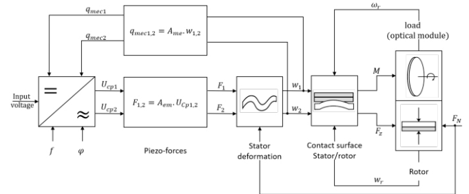
Fig. 9. Block diagram of traveling wave piezoelectric motor (Bullo, 2005)
