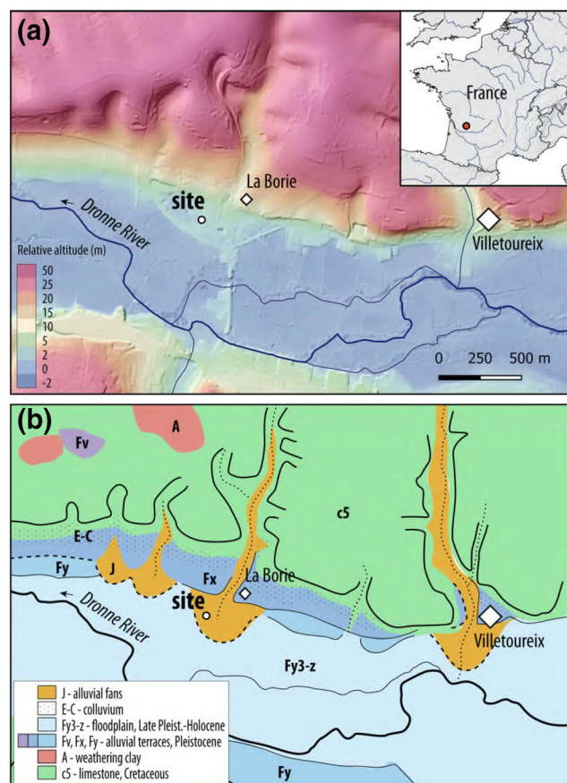
FIGURE 1 Location and geomorphological setting of the study site. A – Topography from Lidar survey (RGEALTI 5 m, Institut Géographique National); B – Geology, modified from the 1:50,000 digital geological map of France ( https://infoterre.brgm.fr/ ). The labels of geological units are from Bourbon. 20 In (B), the longitudinal slope of the river has been subtracted from the digital elevation model, and the values indicated are altitudes relative to the riverbanks.
