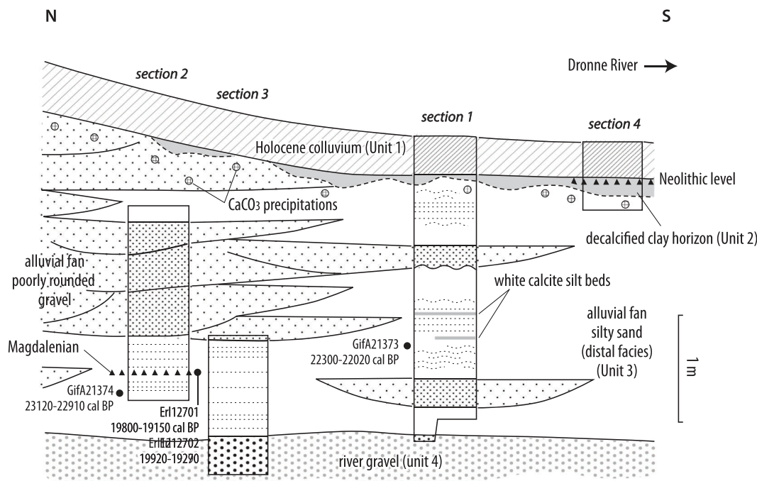
FIGURE 4 Synthetic cross-section of the site. GifA2137-: Radiocarbon age, this study; Erl1270-: Radiocarbon age from Chancelrel. 21
