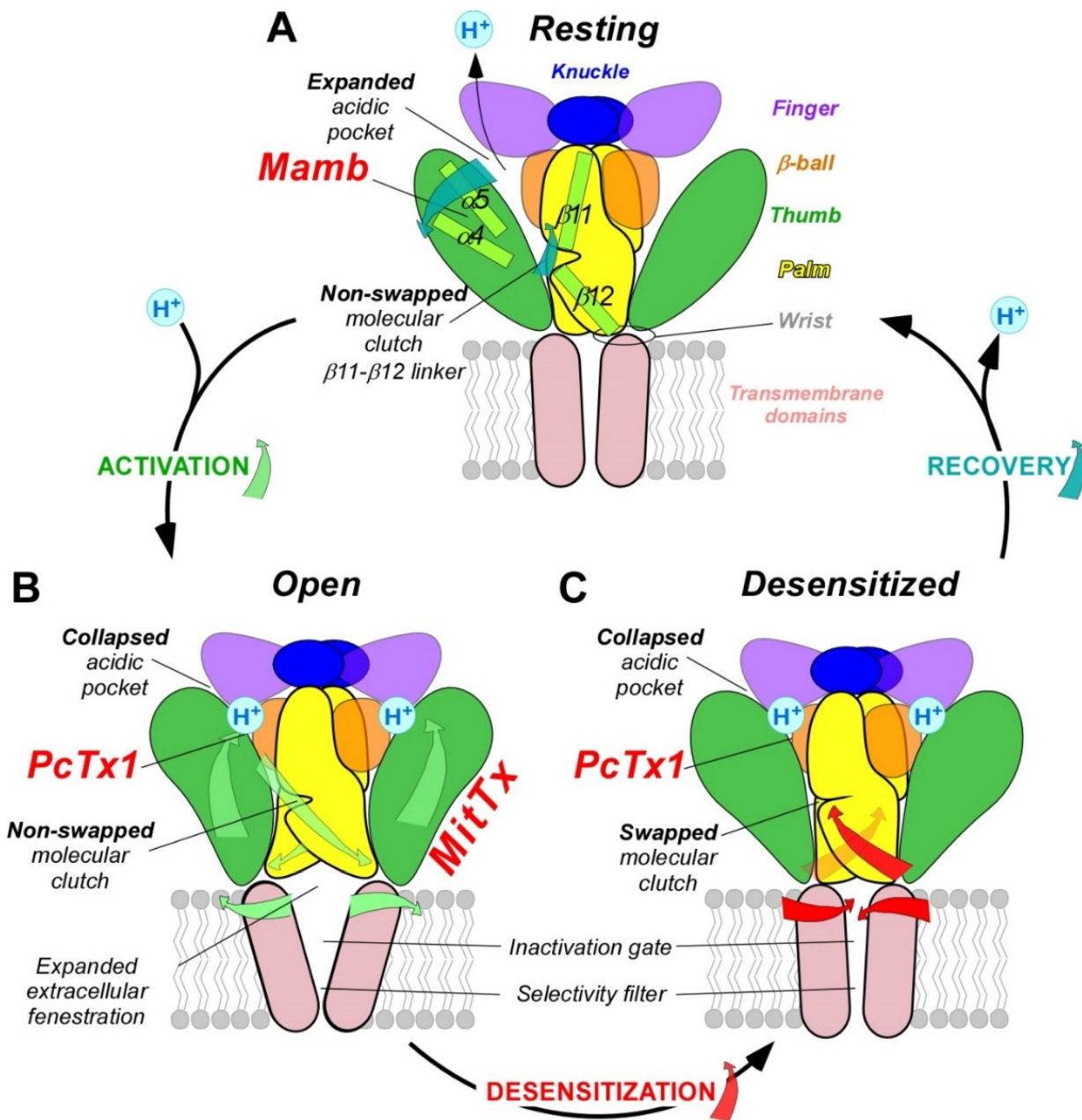
Figure 3. pH-dependent gating mechanisms of ASICs and interaction with toxins. ASIC gating involves three conformational states. (A) , high pH resting state, which is stabilized by the snake toxin mambalgin (major domains involved are indicated with the same color code as in Figure 1 ). (B) , low pH open state, which is stabilized by the snake toxin MitTx and also partially by the spider toxin PcTx1. (C) , low pH desensitized state also promoted by PcTx1. To illustrate the recovery process in (A) , the deprotonation mechanism of only one acidic pocket is presented. Blue (A) , green (B) and red (C) arrows show critical conformational changes during recovery, activation and desensitization processes, respectively. For clarity, only two subunits are shown.
