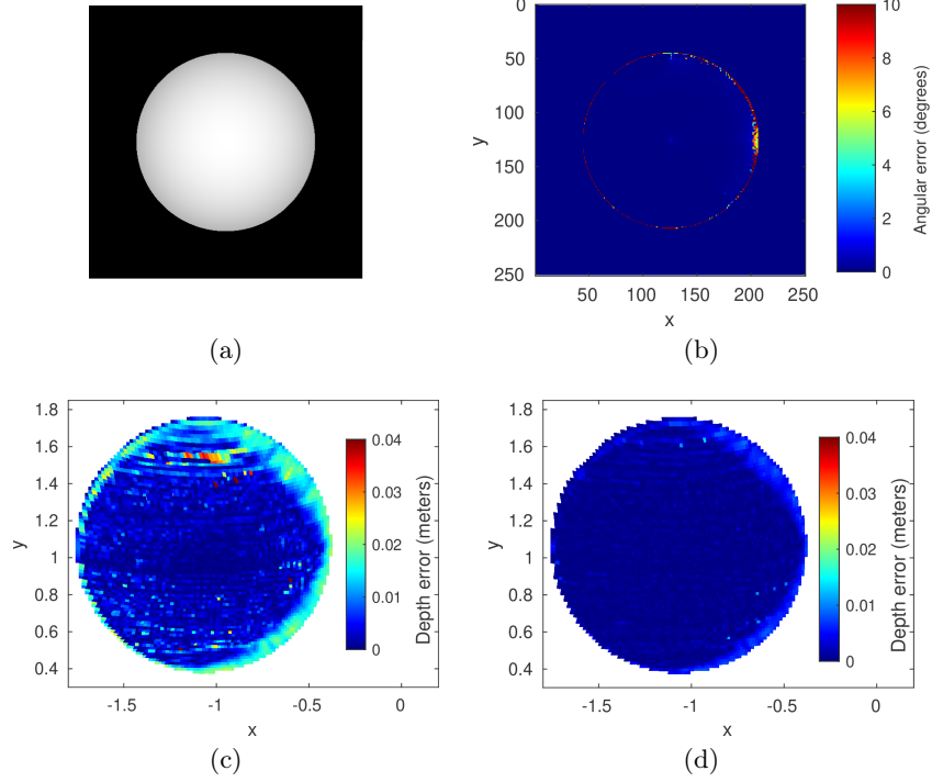
Fig. 3. (a) Reference view. (b) Angular error (in degrees) between the normal estimated according to the method described in Section 3 and the ground truth. (c) Depth error resulting from standard plane-sweeping, using a fronto-parallel patch. (d) Depth error resulting from the proposed slanted plane-sweeping, using a patch oriented according to the estimated normal. The proposed method is globally more accurate.
