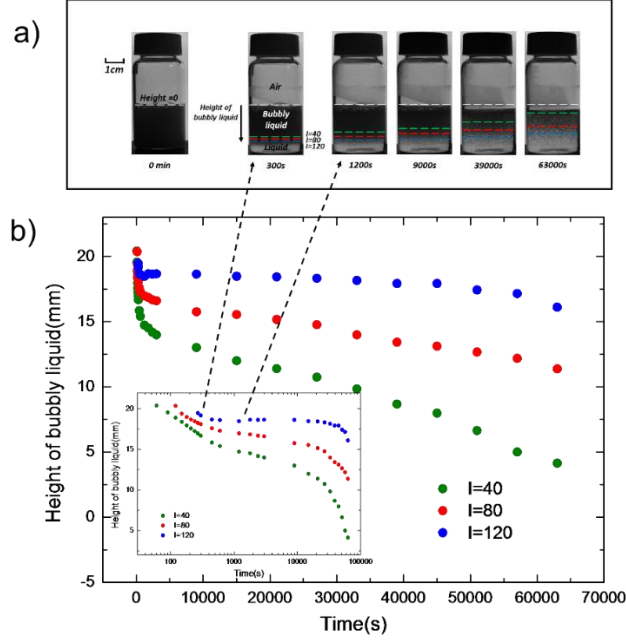
Figure 4. (a) Images of the bottles containing bubbly liquids at different times, showing the front evolution at the different intensity levels I = 40 (green), 80 (red) and 120 (blue). The white line indicates the level of the bubbly liquid at the beginning of the experiment. (b) Height of bubbly liquid versus time for different grey levels. The inset is a semi-logarithmic plot. The system shown in the image is a solution with 20\text{mM} CTAB and 13\text{ mM} NaSal at \varphi_{gas} = 5\% .
