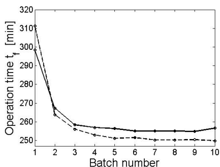
Figure 2. Evolution of final batch time. Case I: solid, Case II: dashed.
