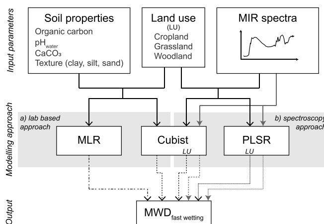
Fig. 2. Modelling approaches followed in this study for the prediction of the aggregate stability.
