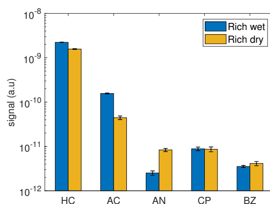
Figure 4. Observed average signal of VOCs during an isothermal experiment at the maximum observed signal (280 °C) for R and R-H 2 O gas mixtures (HC: hydrocarbons m/z 41; AC: acetone; AN: acrylonitrile; CP: cyanopropene; BZ: benzene) for rich conditions in a wet (H 2 O 3%) or dry (H 2 O 0%) environment. Measurements were performed with a MS equipped with a membrane for MIMS analysis.
