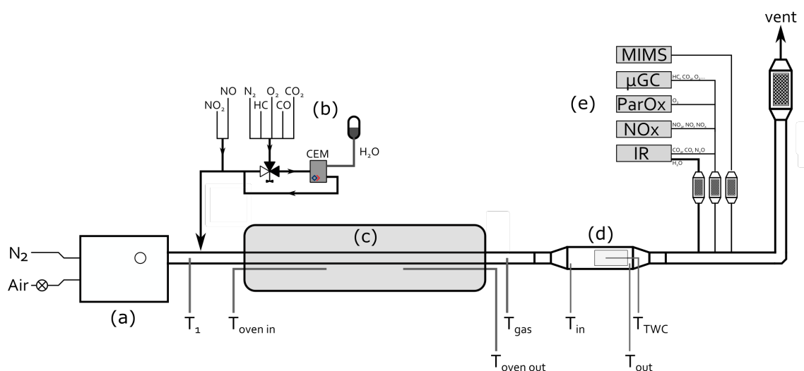
Figure 6. Synthetic gas bench (SGB) scheme: (a) nitrogen stream generator, (b) gas-lines mixing system (CO, NO, O 2 , CO 2 , HC) with a water evaporator (CEM), (c) pre-heating oven, (d) reactor with inserted TWC, (e) analyzers (MIMS: membrane inlet mass spectrometer; µGC: micro gas chromatograph; ParOx: paramagnetic oxygen analyzer; NO x : Chemiluminescence (two inlets) NO, NO 2 , NO x analyzer; online IR (heated line) infrared analyzer for CO, N 2 O, CO 2 , H 2 O). Temperature and flowmeter are controlled by a LabView software.
