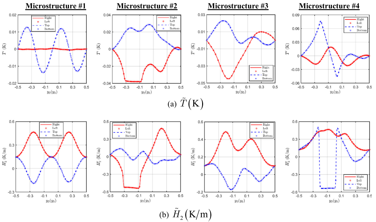
Fig. 20. Comparison of fluctuating temperature and its gradients along the unit cell boundaries, illustrating the exact satisfaction of periodicity boundary conditions.
