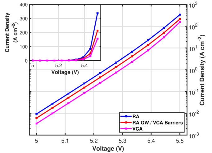
FIG. 2. (a) Current-voltage curves, on a log-scale, for an \text{Al}_{0.7}\text{Ga}_{0.3}\text{N}/\text{Al}_{0.8}\text{Ga}_{0.2}\text{N} quantum well embedded in a p - n junction. The data are shown for simulations that (i) account for random alloy (RA) fluctuations in the well and barriers (blue), (ii) account for RA fluctuations in the well but treat the barrier in a virtual crystal approximation (VCA) (red), and (iii) use a VCA in the entire p - i - n structure (pink). The inset shows the I-V curves on a linear scale.
